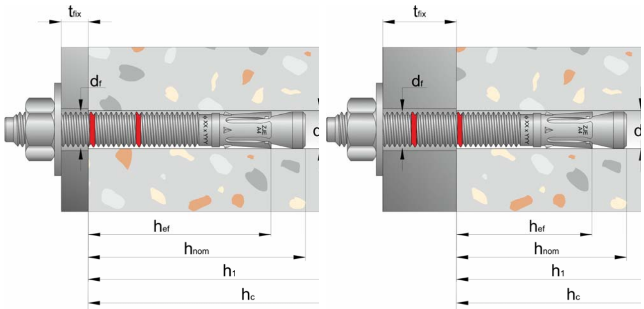
Reduced embedment depth (sizes M8, M10, M12, M16 and M20)
